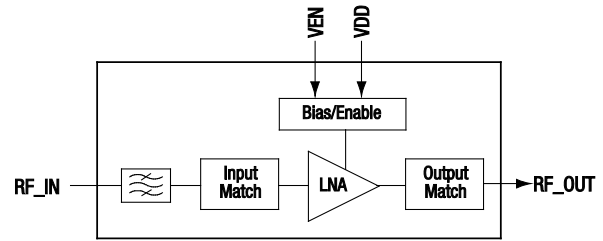
Figure 1. SKY65709-51 Block Diagram
