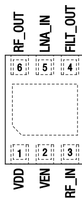
Figure 2. SKY65709-51 Pinout – 6-Pin MCM (Top View)
