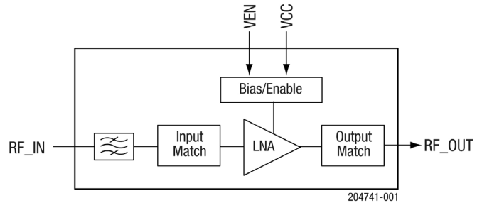
Figure 1. SKY65728-11 Block Diagram
