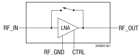
Figure 1. SKY65804-696LF Block Diagram
