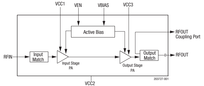
Figure 1. SKY66188-11 Linear PA Block Diagram
