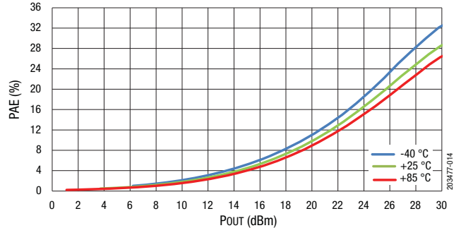
Figure 14. Power-Added Efficiency vs Output Power @ 5200 MHz
