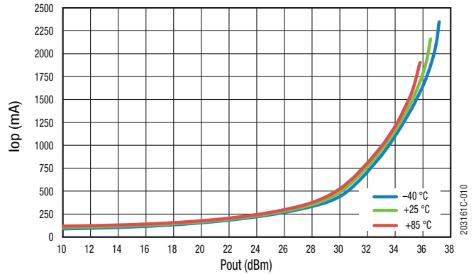
Figure 10. Operating Current vs Pout Across Temperature
