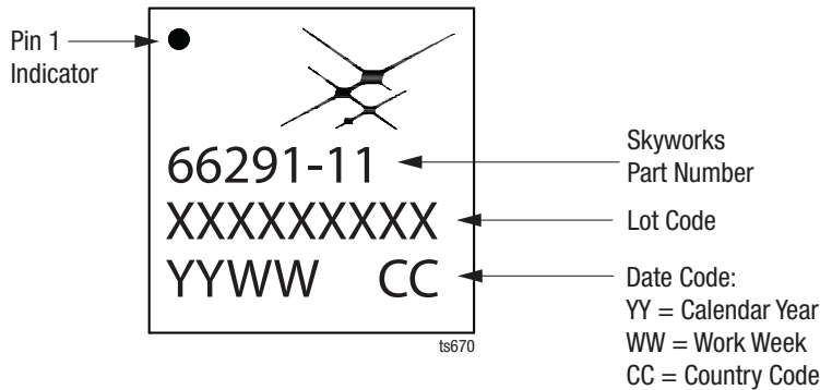
Figure 21. Typical Part Marking for the SKY66291-11
