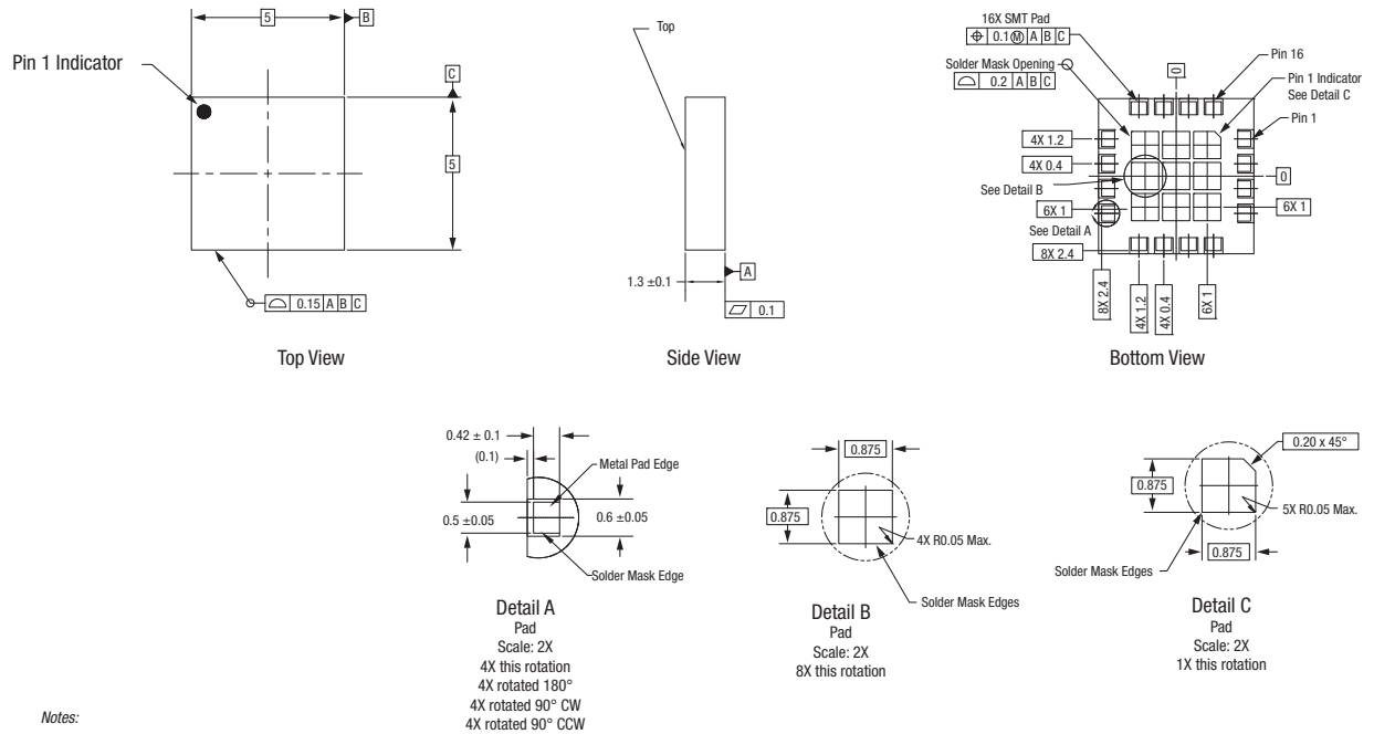
Figure 23. SKY66295-11 Package Dimensions
