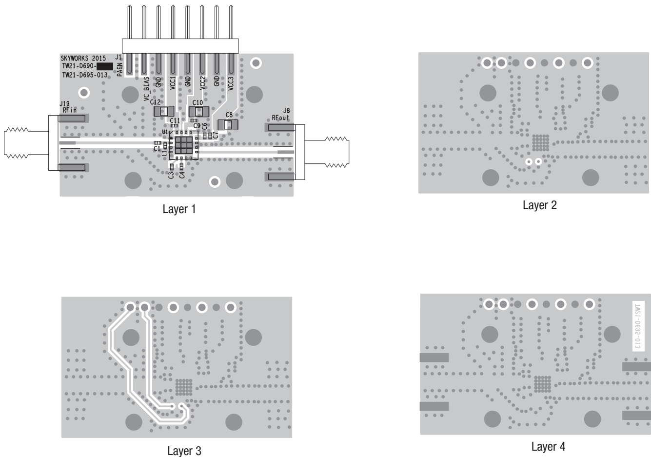
Figure 19. Evaluation Board Layer Details
