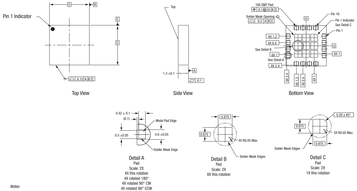
Figure 23. SKY66297-11 Package Dimensions
