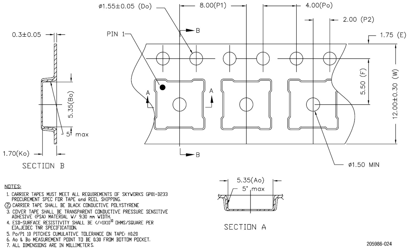
Figure 24. SKY66318-11 Tape and Reel Dimensions
