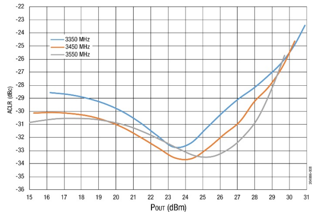
Figure 8. ACLR (5x20MHz) vs Pout Across Frequency
