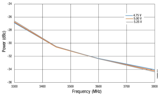
Figure 13. 2nd Harmonic vs Frequency Across Voltage (Pout = +28 dBm, CW)
