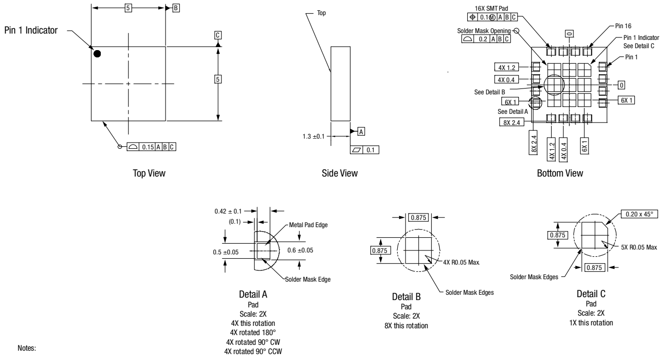
Figure 23. SKY66391-12 Package Dimensions
