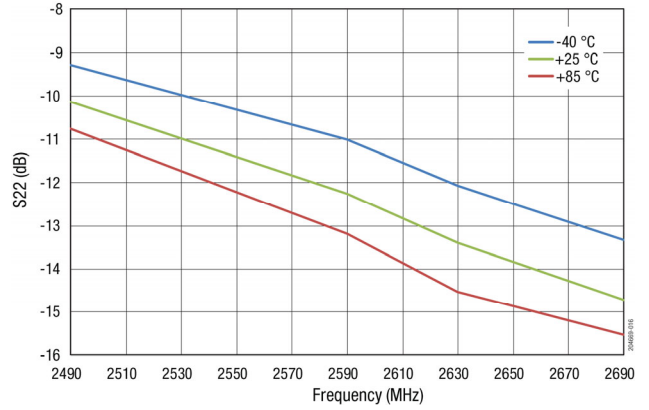
Figure 16. S22 vs Frequency Across Temperature (PIN = -20 dBm)
