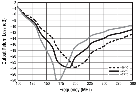
Figure 7. Small Signal Output Return Loss (IS22) vs Frequency and Temperature, Narrow Band
