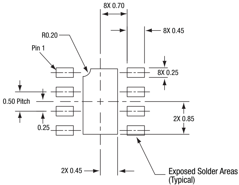
Figure 17. SKY67100-396LF PCB Layout Footprint (Top View)
