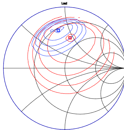
Figure 18. OIP3 Load Pull @ 0.45 GHz, 5 V, 76 mA (Input Load = NF Min., -20 dBm/Tone, 5 MHz Spacing)
