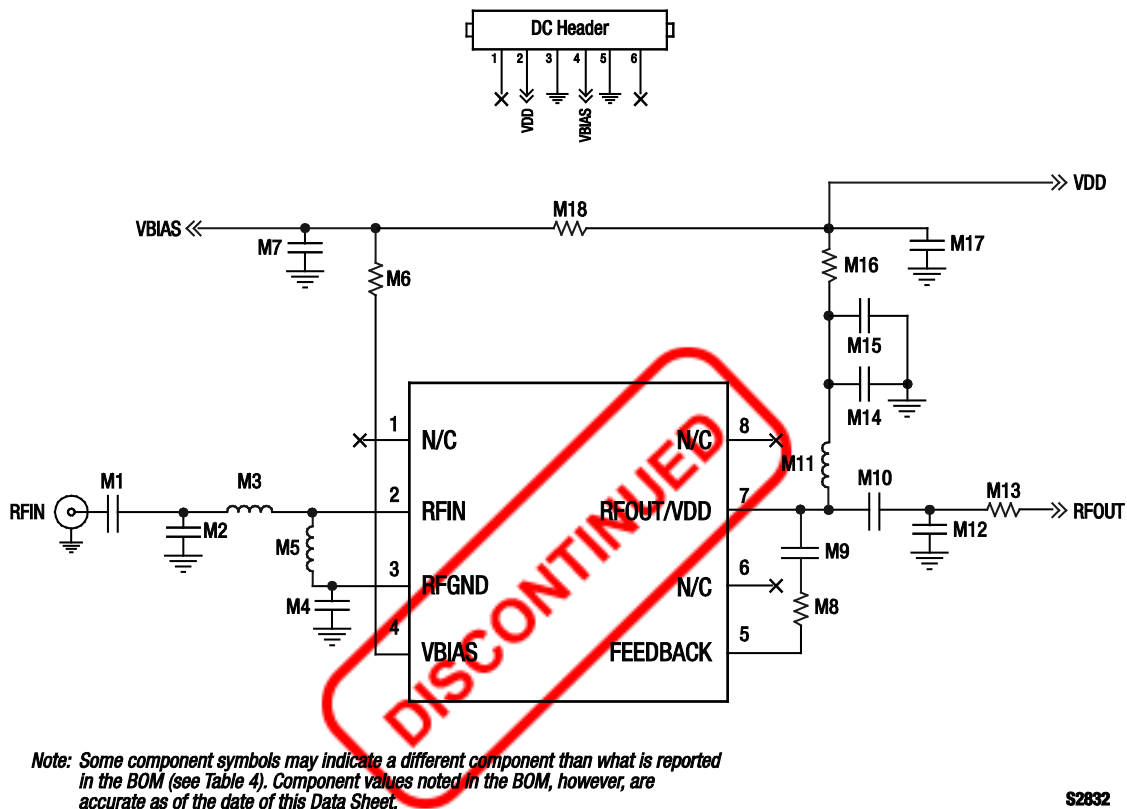
Figure 21. SKY67110-396LF Evaluation Board Schematic
