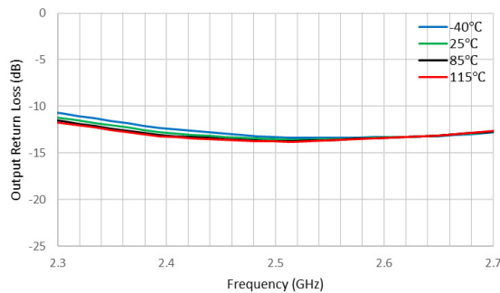
Figure 20. Output Return Loss (dB) vs Frequency
