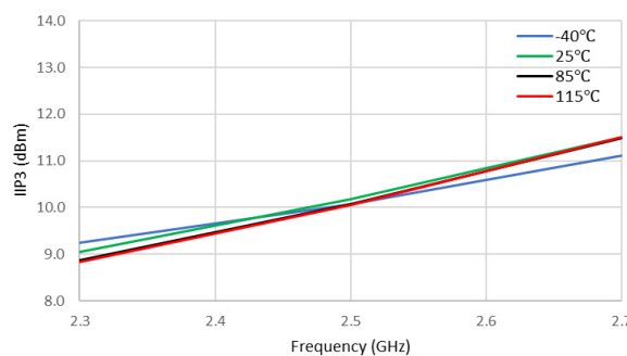
Figure 22. IIP3 (dBm) vs Frequency (GHz)
