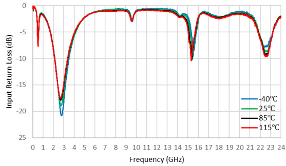
Figure 26. Input Return Loss (dB) vs Frequency (GHz)
