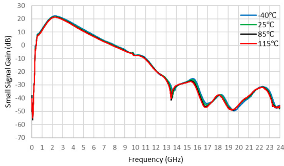
Figure 25. Small Signal Gain (dB) vs Frequency (GHz)
