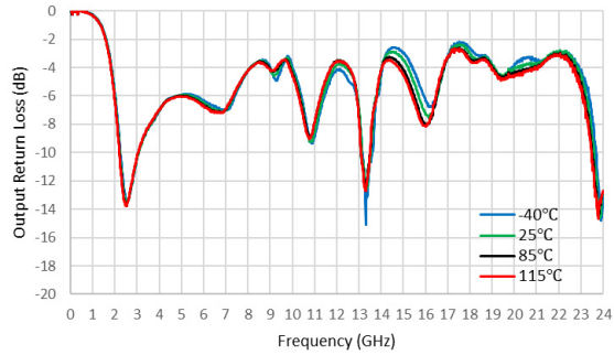
Figure 28. Output Return Loss (dB) vs Frequency (GHz)
