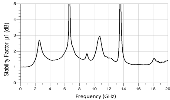
Figure 29. Stability Factor, \mu_1 (dB) vs Frequency (GHz) at -40 °C
