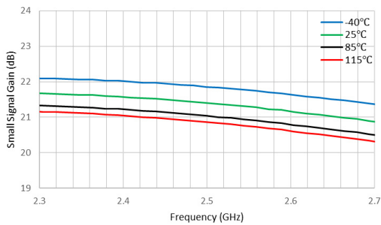
Figure 17. Small Signal Gain (dB) vs Frequency (GHz)
