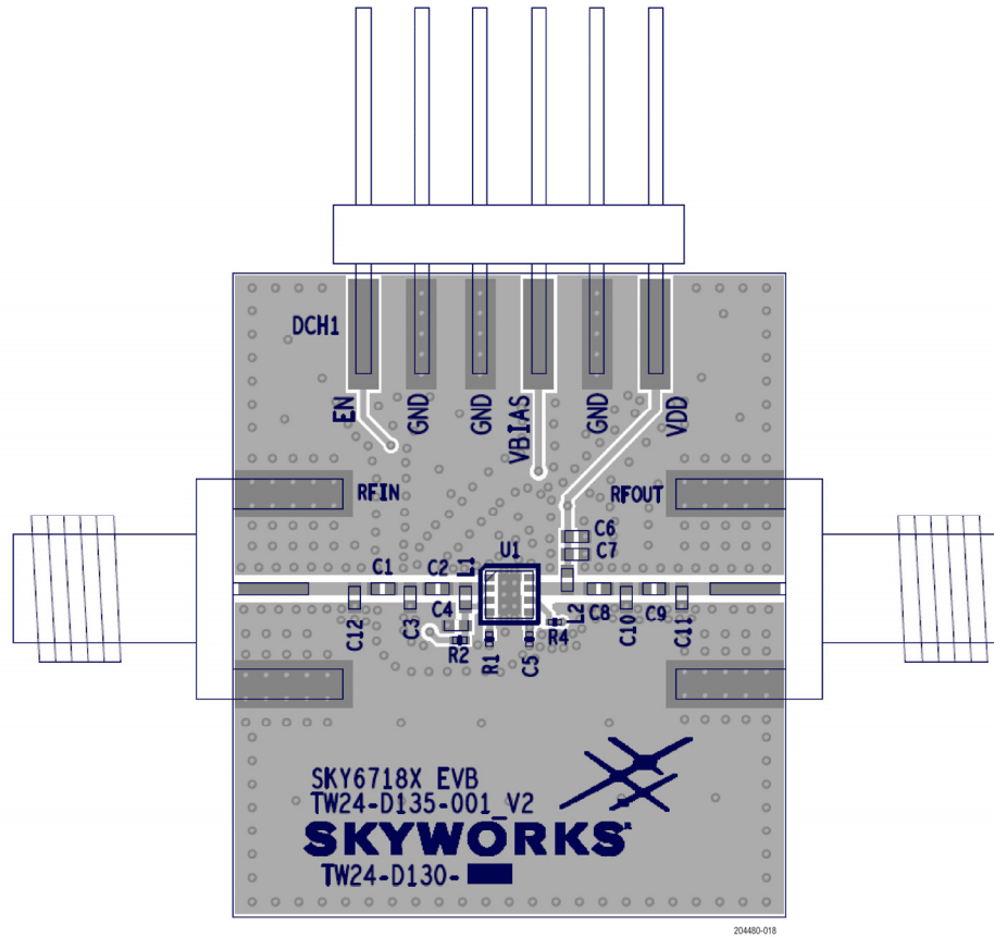
Figure 46. SKY67183-396LF EVB Assembly Diagram
