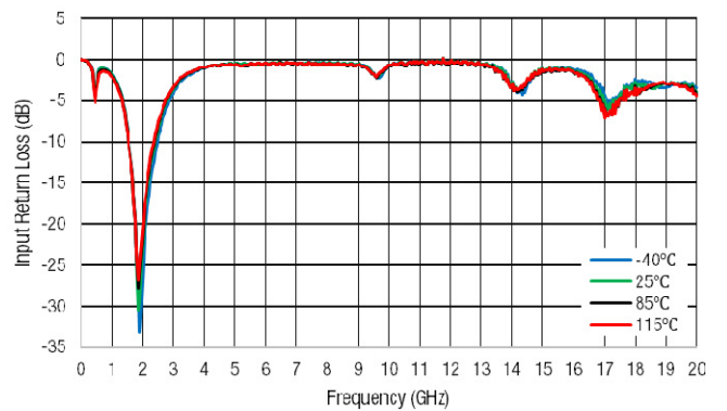
Figure 40. Input Return Loss (dB) vs Frequency (GHz)
