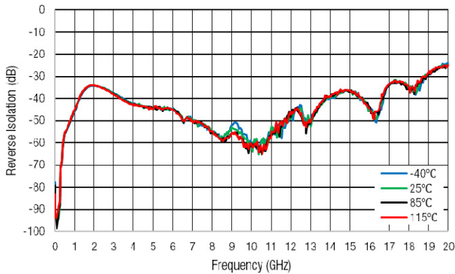
Figure 41. Reverse Isolation (dB) vs Frequency (GHz)
