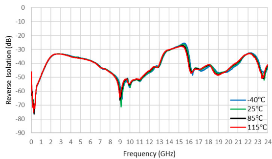
Figure 27. Reverse Isolation (dB) vs Frequency (GHz)
