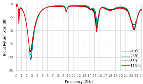
Figure 26. Input Return Loss (dB) vs Frequency (GHz)
