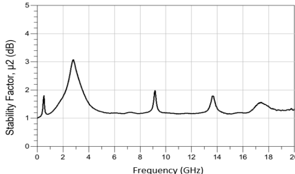
Figure 30. Stability Factor, \mu_2 (dB) vs Frequency (GHz) at -40 °C
