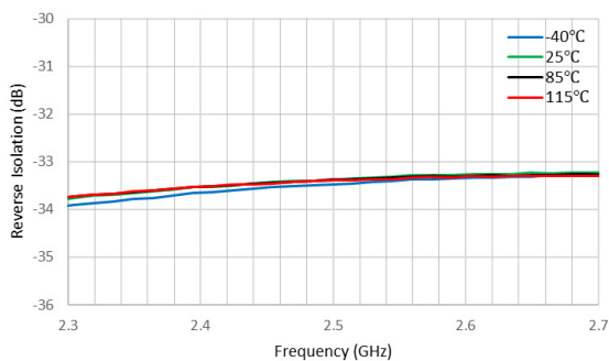
Figure 21. Reverse Isolation (dB) vs Frequency (GHz)
