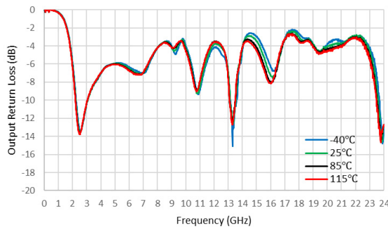
Figure 28. Output Return Loss (dB) vs Frequency (GHz)
