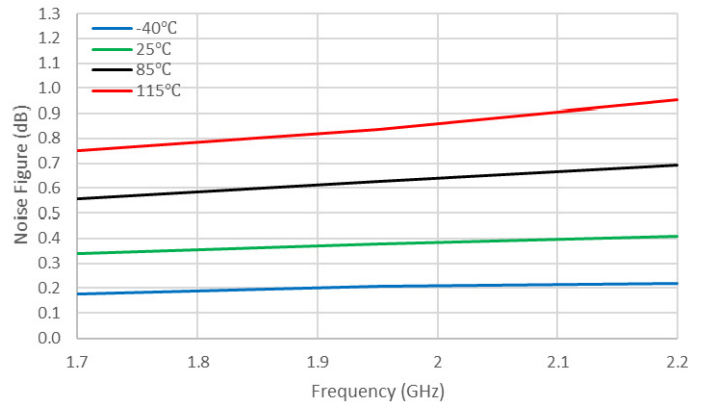
Figure 32. Noise Figure (dB) vs Frequency (GHz)
