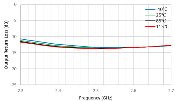
Figure 20. Output Return Loss (dB) vs Frequency
