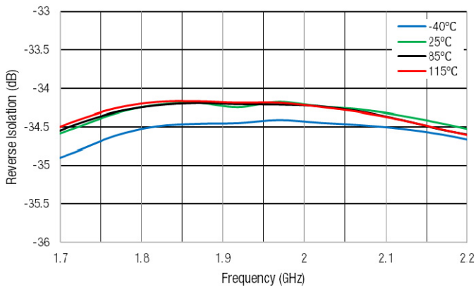
Figure 35. Reverse Isolation (dB) vs Frequency (GHz)
