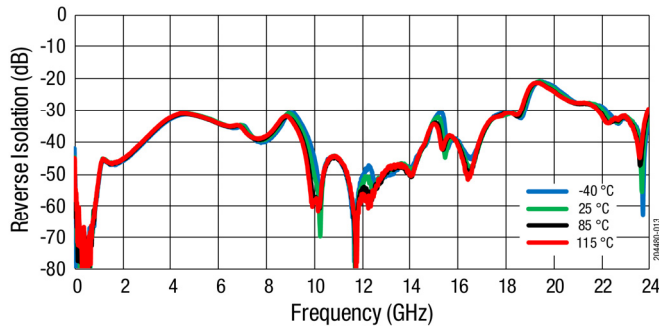
Figure 13. Reverse Isolation (dB) vs Frequency (GHz)
