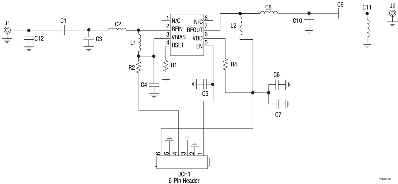
Figure 45. SKY67183-396LF Evaluation Board Schematic
