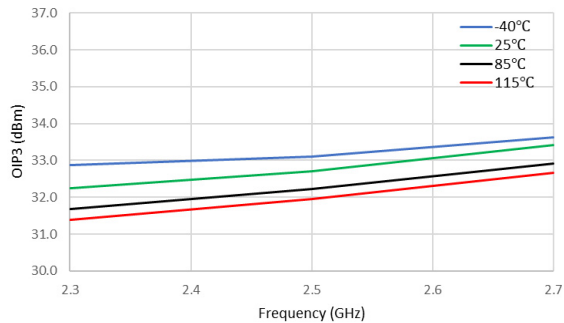
Figure 23. OIP3 (dBm) vs Frequency (GHz)
