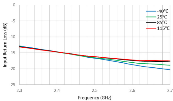
Figure 19. Input Return Loss (dB) vs Frequency
