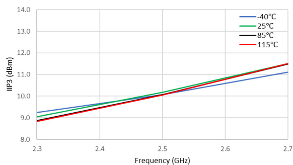
Figure 22. IIP3 (dBm) vs Frequency (GHz)
