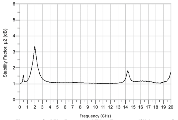
Figure 44. Stability Factor, \mu_2 (dB) vs Frequency (GHz) at -40 °C
