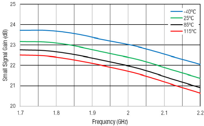
Figure 31. Small Signal Gain (dB) vs Frequency (GHz)
