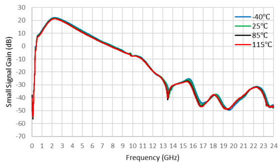
Figure 25. Small Signal Gain (dB) vs Frequency (GHz)
