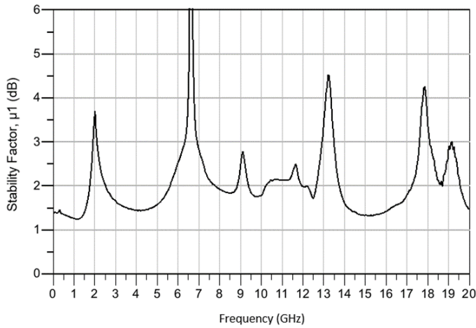
Figure 43. Stability Factor, \mu_1 (dB) vs Frequency (GHz) at -40 °C
