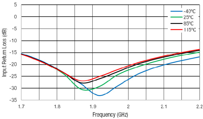
Figure 33. Input Return Loss (dB) vs Frequency
