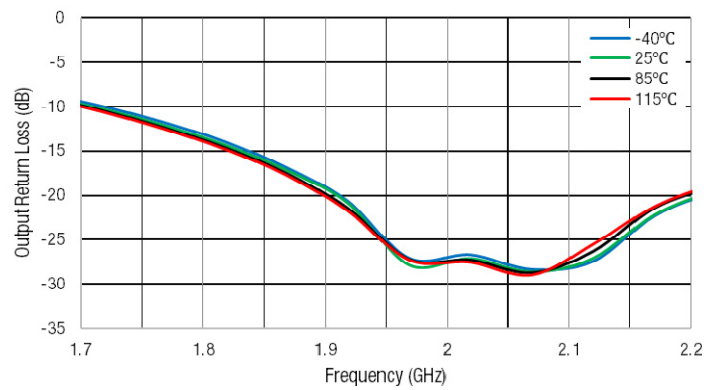
Figure 34. Output Return Loss (dB) vs Frequency
