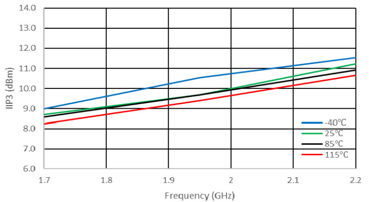
Figure 36. IIP3 (dBm) vs Frequency (GHz)
