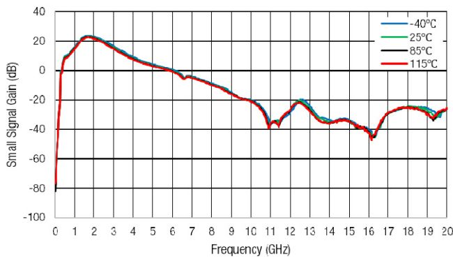
Figure 39. Small Signal Gain (dB) vs Frequency (GHz)
