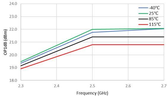
Figure 24. OP1dB (dBm) vs Frequency (GHz)
