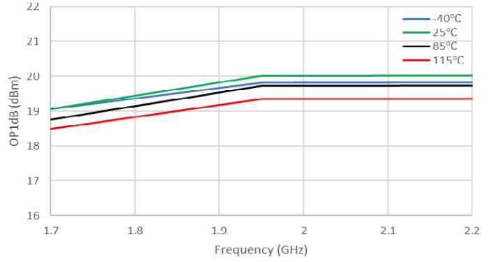
Figure 38. OP1dB (dBm) vs Frequency (GHz)
