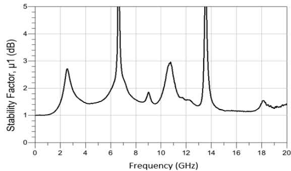
Figure 29. Stability Factor, \mu_1 (dB) vs Frequency (GHz) at -40 °C
