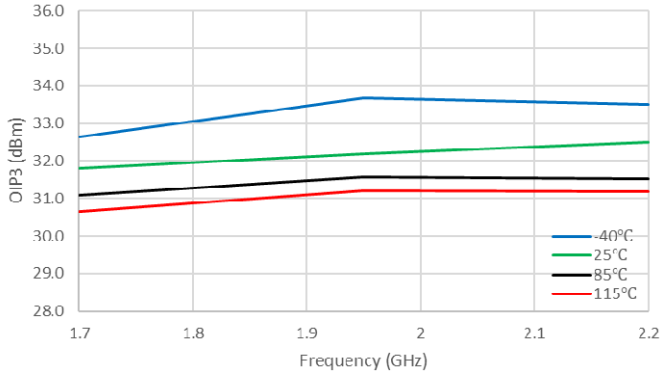
Figure 37. OIP3 (dBm) vs Frequency (GHz)
