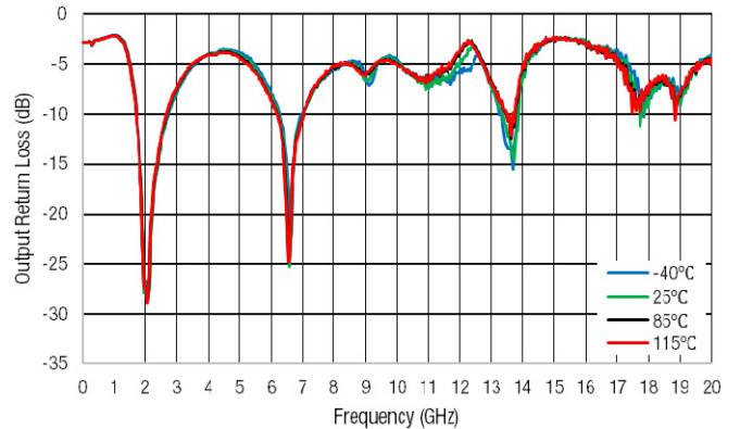
Figure 42. Output Return Loss (dB) vs Frequency (GHz)
