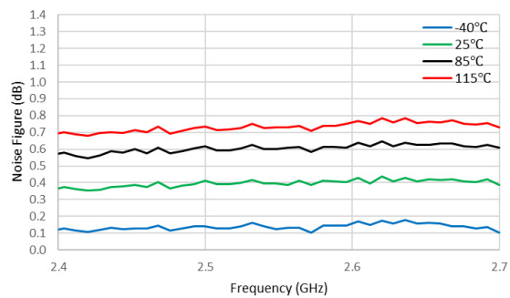
Figure 18. Noise Figure (dB) vs Frequency (GHz)
