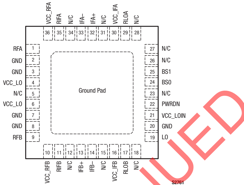
Figure 2. SKY73420-11 Pinout – 36-Pin QFN (Top View)
