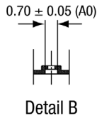
Figure 10. SOD-882 Tape and Reel Dimensions
