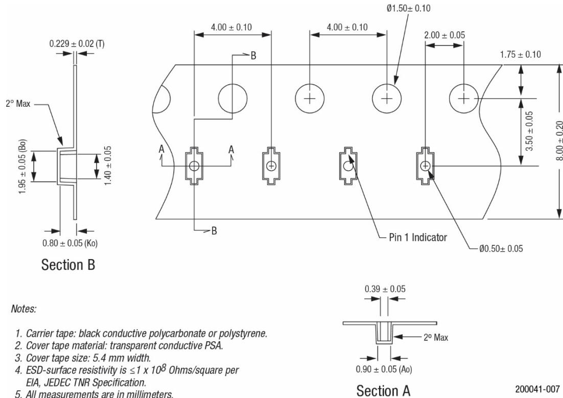
Figure 5. SC-79 Tape and Reel Dimensions
