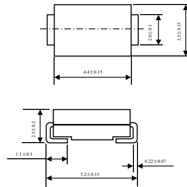
1.5WATT SURFACE MOUNTSILICON ZENER DIODES Dimensions in inches and (millimeters)
