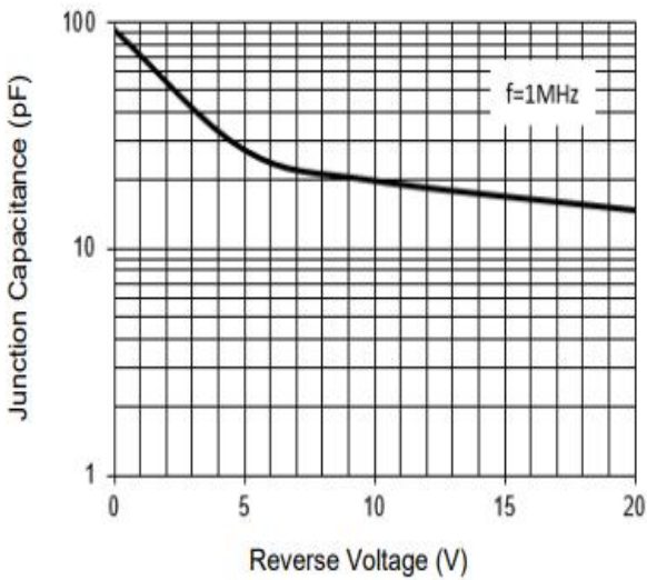
Fig 3. Junction Capacitance
