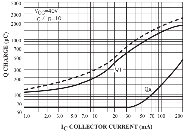
Figure 4. Charge Data
