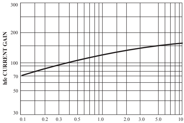
Figure 11. Current Gain
