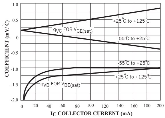
Figure 18. Temperature Coefficients
