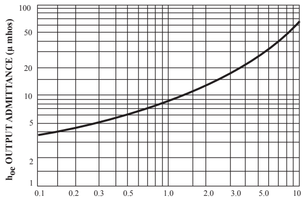
Figure 12. Output Admittance
