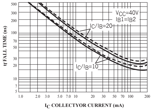
Figure 24. Fall Time
