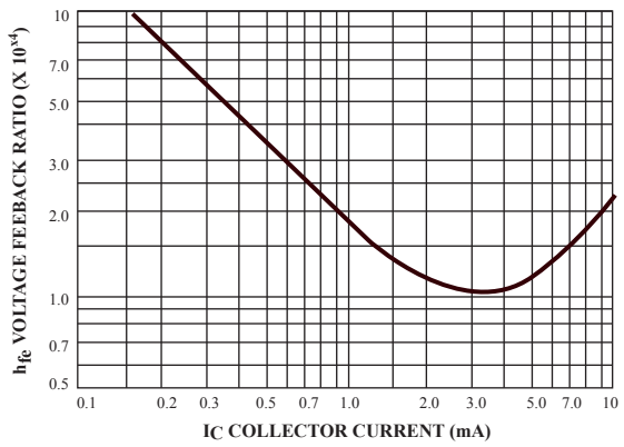
Figure 30. Votage Feedback Ratio
