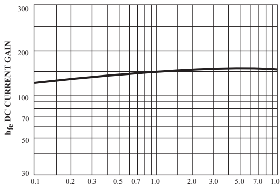
Figure 27. Current Gain
