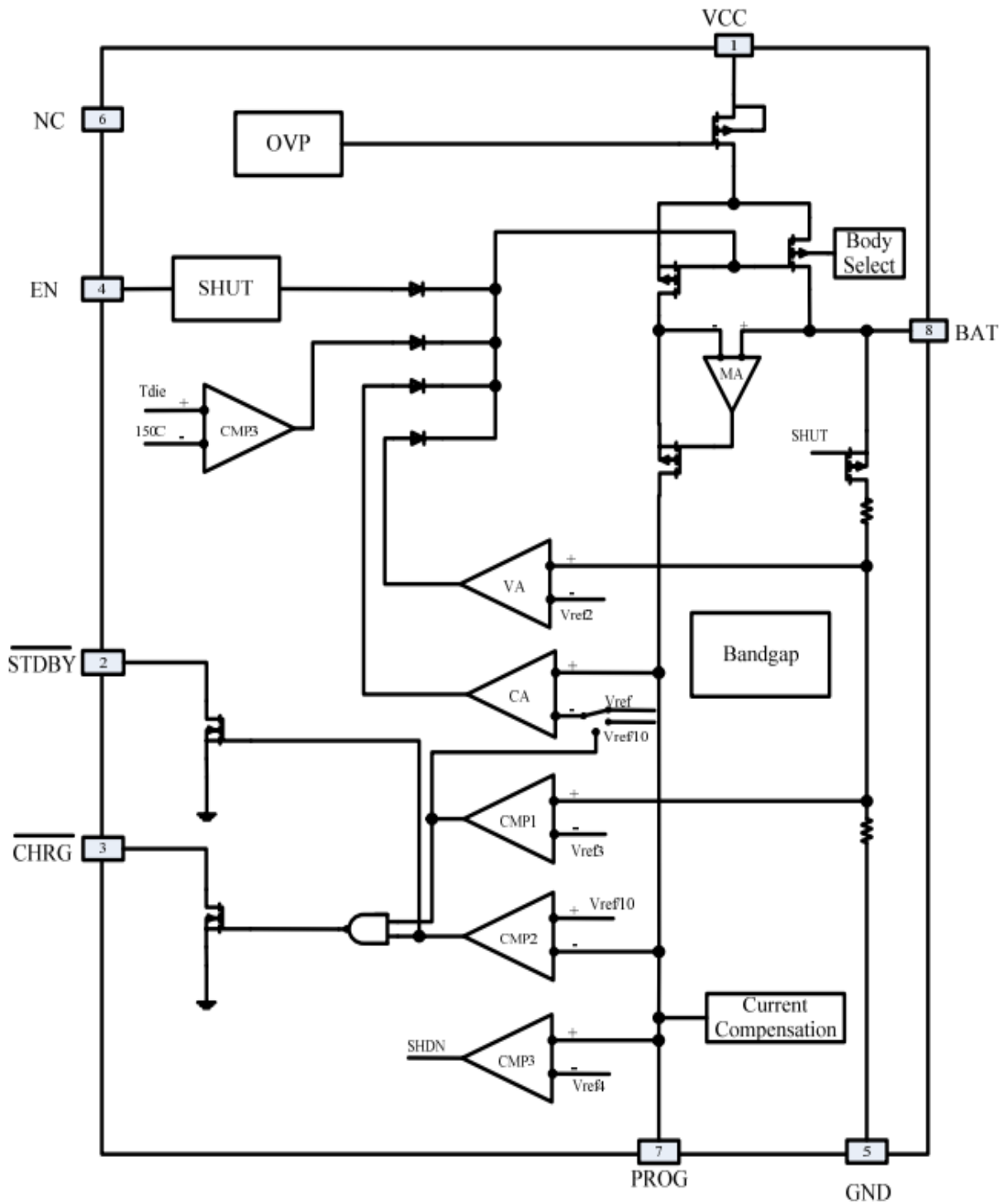
Figure3 Block Diagram
