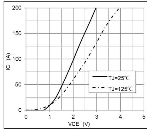
Typical Saturation Voltage Characteristics V GE =15V
