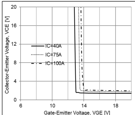
Saturation Voltage vs. VGE T c =25 °C
