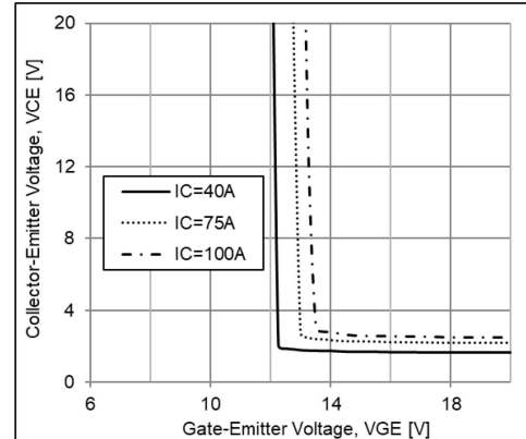
Saturation Voltage vs. VGE T c =25 °C
