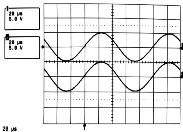
Figure (b) Rail to Rail Capability
