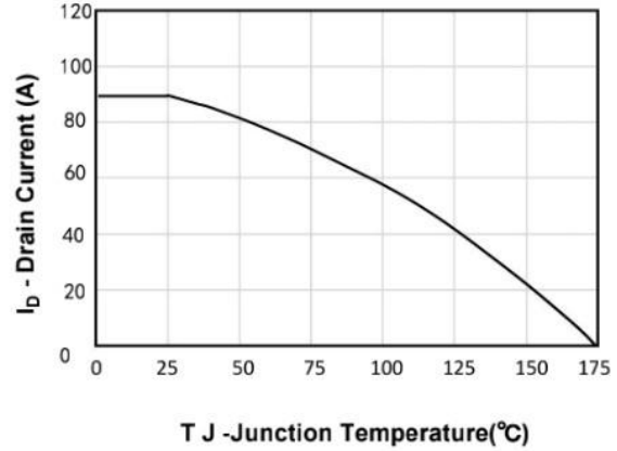
Figure 10. Maximum PContinuous Drain Current vs Case Temperature
