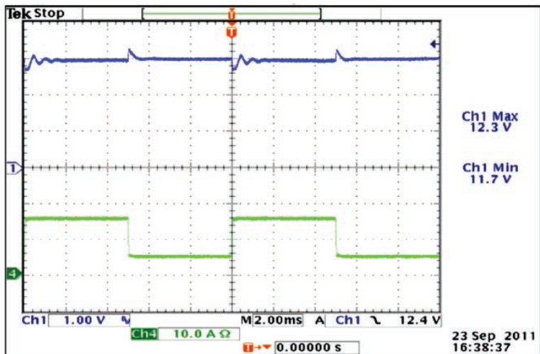
12V OUT, 115VAC, 25% TO 75% LOAD STEP
