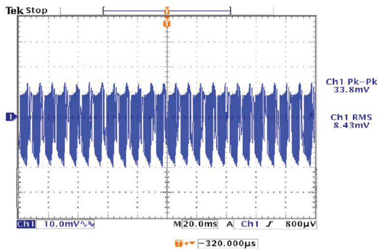
12V Out, No Load, 85VAC, 60HZ
