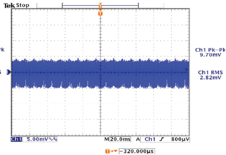
12V Out, No Load, 264VAC, 50HZ
