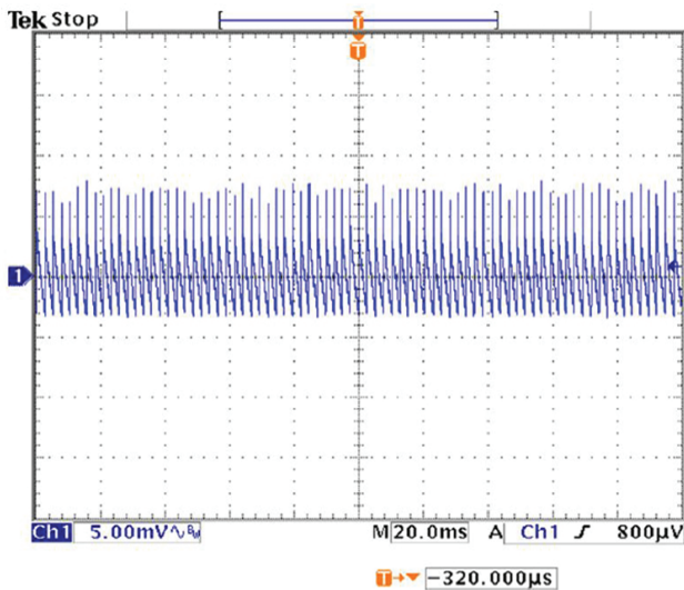
12V Out, No Load, 264VAC, 50HZ
