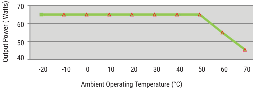
Output Power - Conection vs. Ambient Temperature
