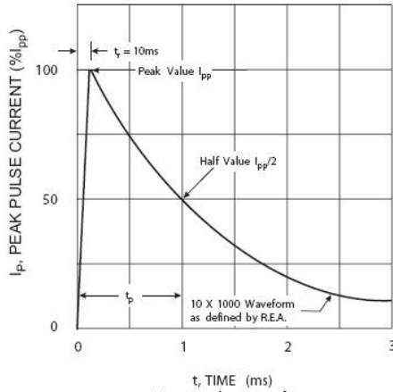
Fig. 1 Pulse Waveform
