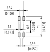
◆ P. C. B LAYOUT
