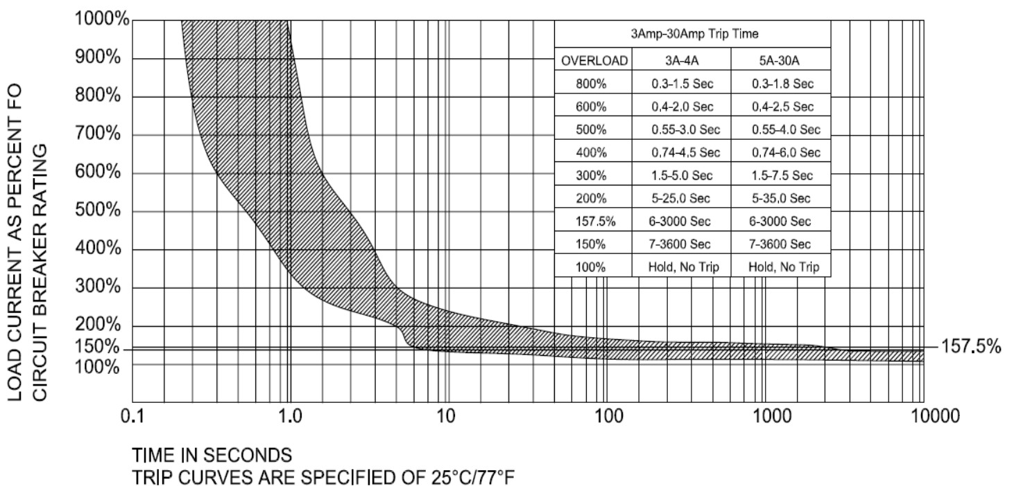
67 SERIES THERMAL CIRCUIT BREAKER TRIP TIME CURVES
