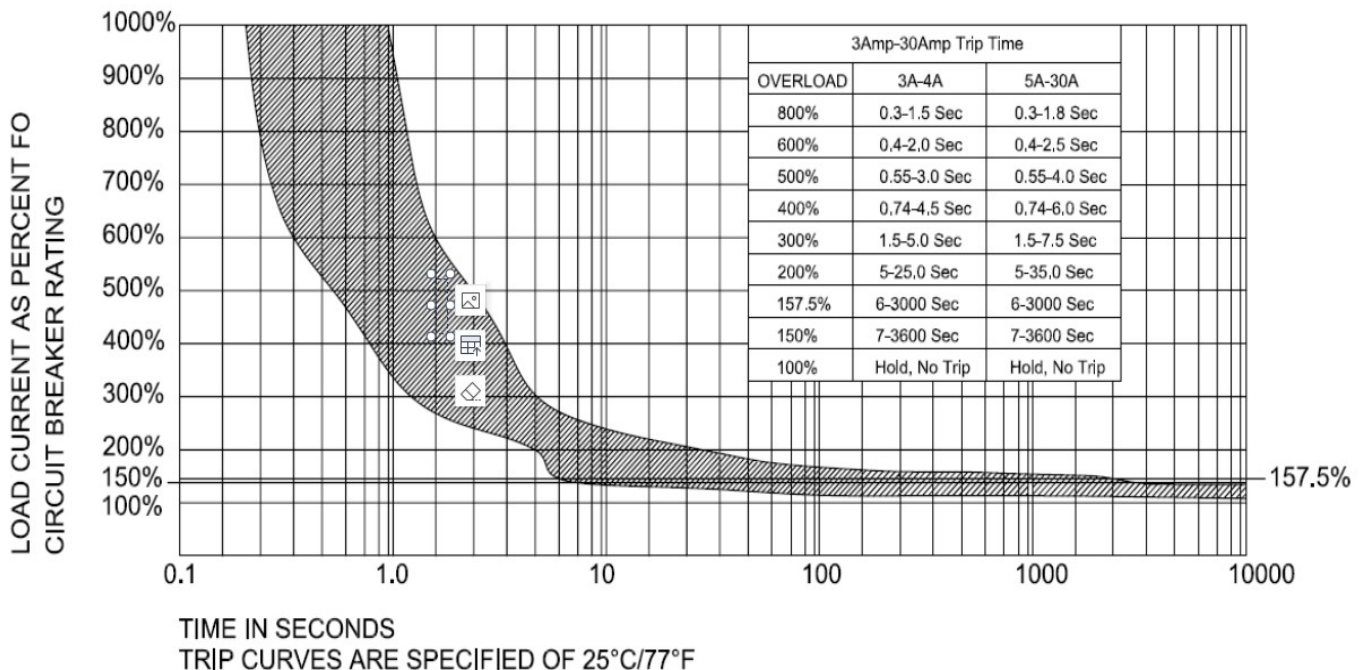
67 SERIES THERMAL CIRCUIT BREAKER TRIP TIME CURVES
