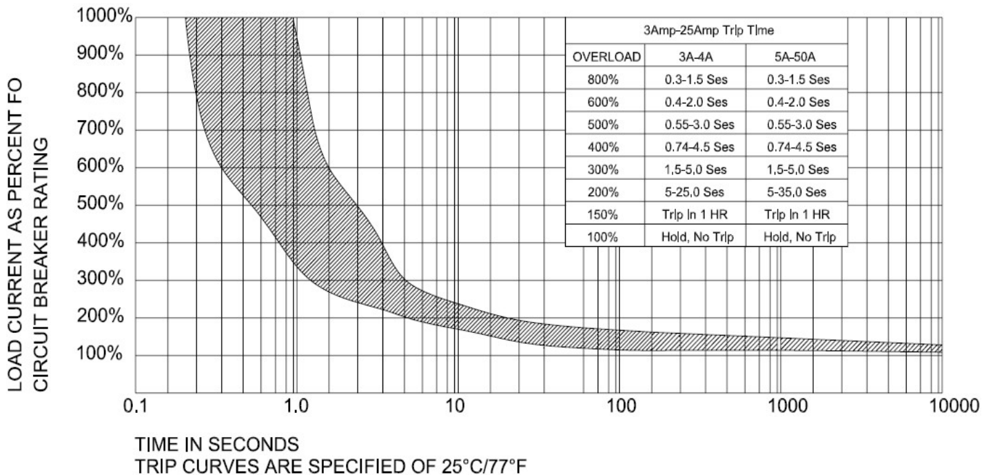
67AR SERIES THERMAL CIRCUIT BREAKER TRIP TIME CURVES
