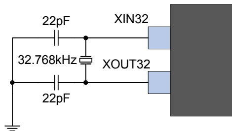
Figure 38-8. External Real Time Oscillator with Load Capacitor
