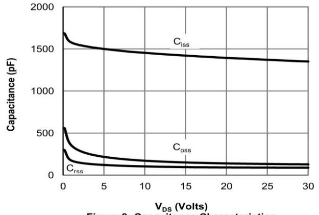
Figure 8: Capacitance Characteristics
