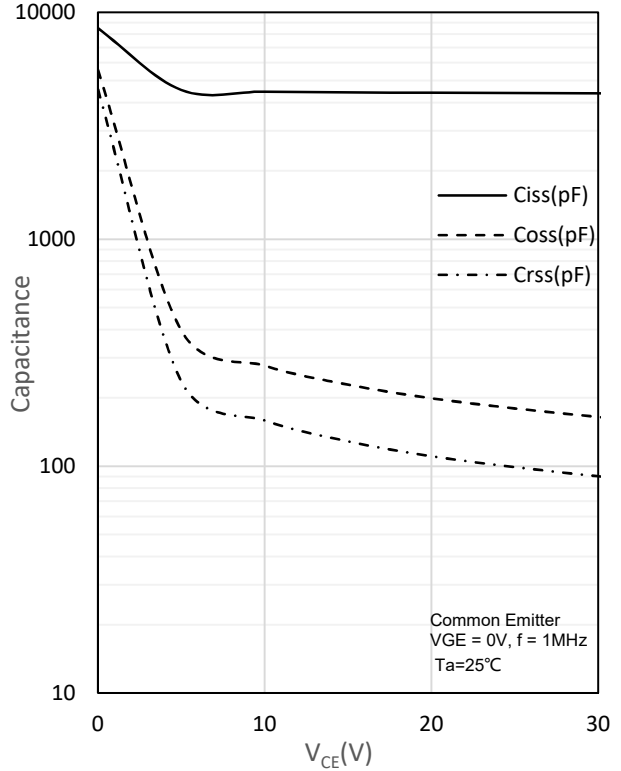
Fig. 12 Capacitance characteristics
