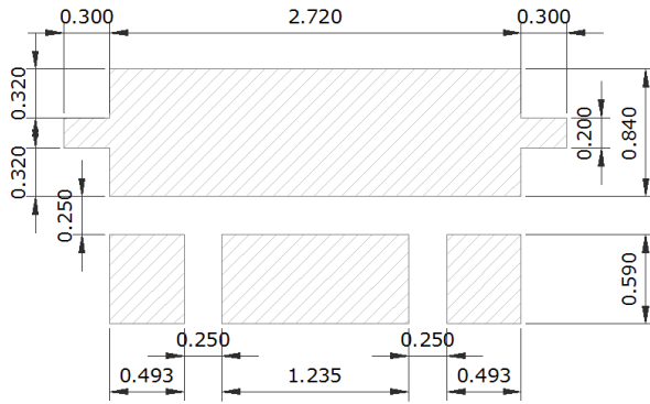
Solder Pad
