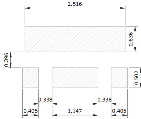
Solder Metal Mask
