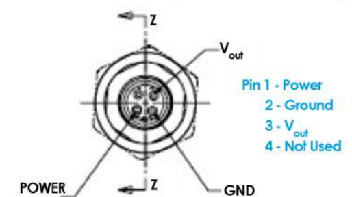
M12 Connector Transducer (1 to 5 Vdc or 0.5 to 4.5 Vdc)
