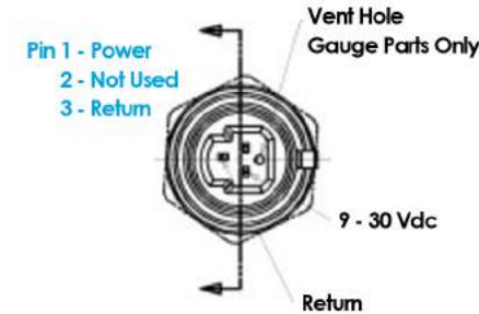
Deutsch Connector Transmitter (4 to 20 mA)
