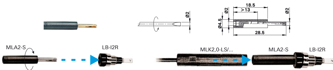
Non-touch-protected socket
