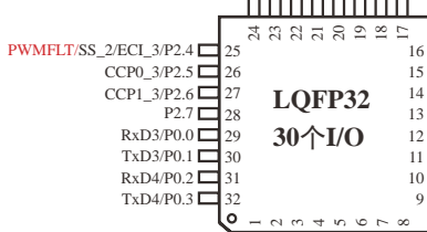
LQFP32 (9x9mm)
