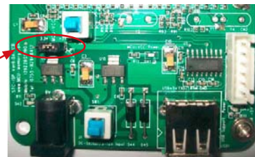
单片机电源电压的选择跳线短接MCU-VCC和5V电源管脚
