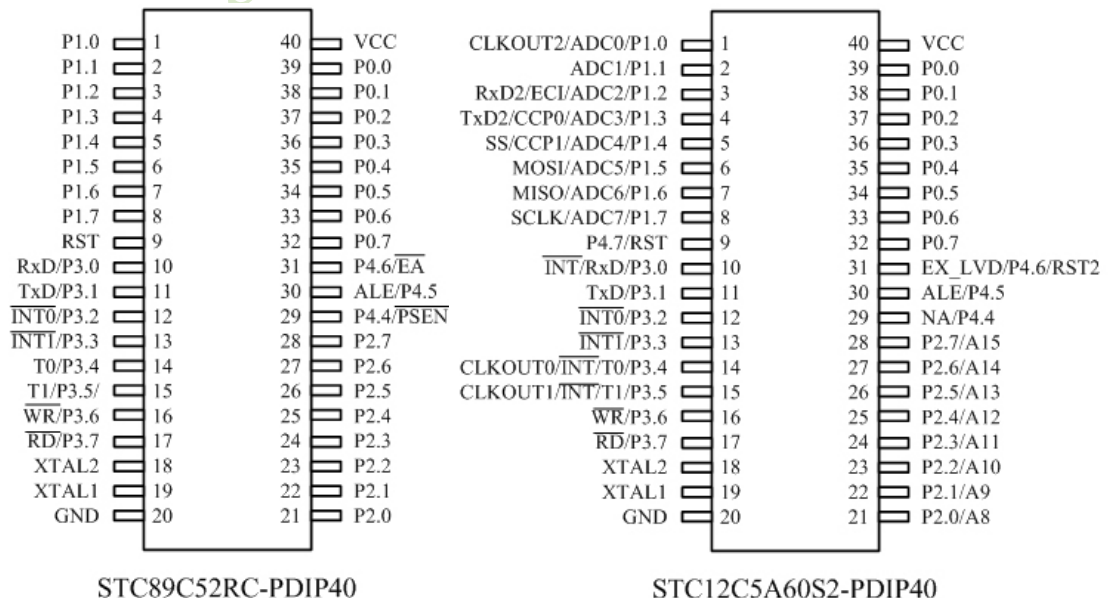
STC89C52RC-PDIP40
