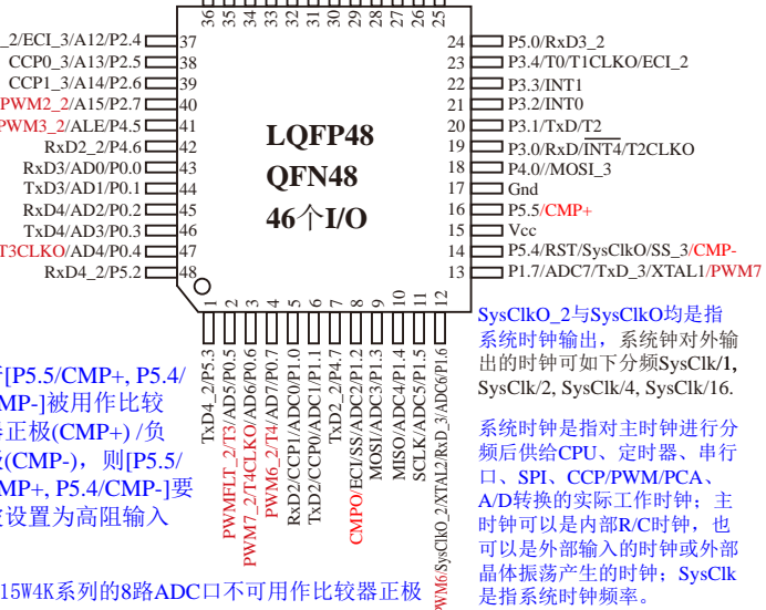
LQFP48 (9x9mm)
