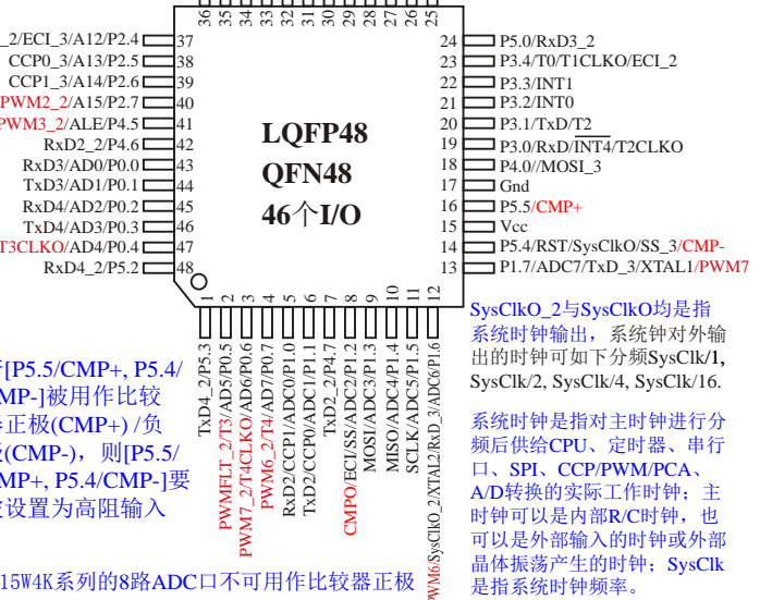
LQFP48 (9x9mm)
