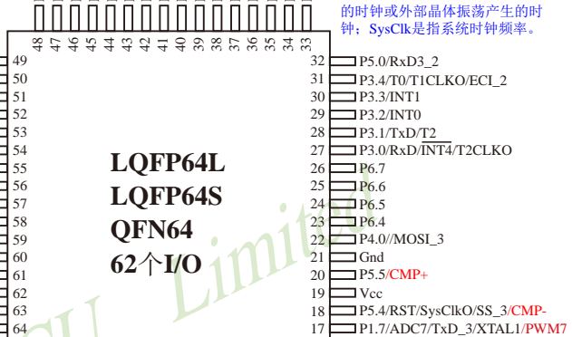
LQFP64L (16mm x 16mm) LQFP64S (12mm x 12mm) QFN64 (9mm x 9mm)
