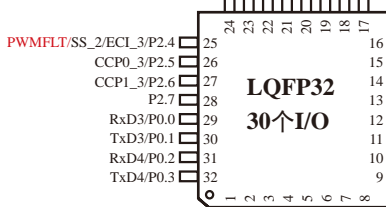
LQFP32 (9x9mm)
