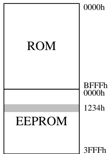
STC32G8K64
