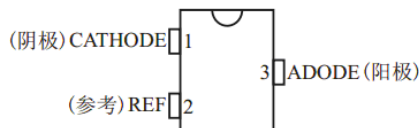
SOT23-3封装, RMB ¥0.15~0.3
