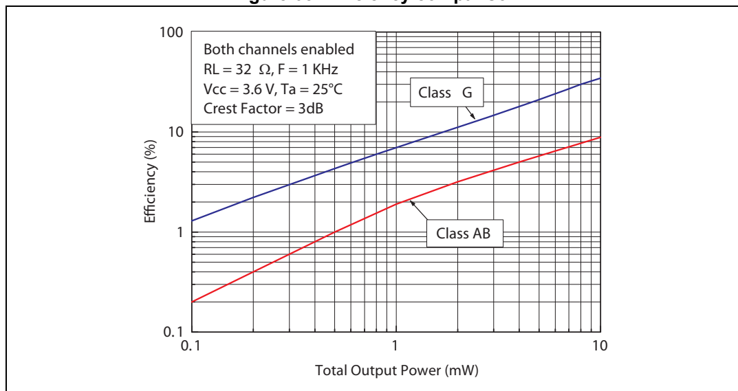
Figure 65. Efficiency comparison
