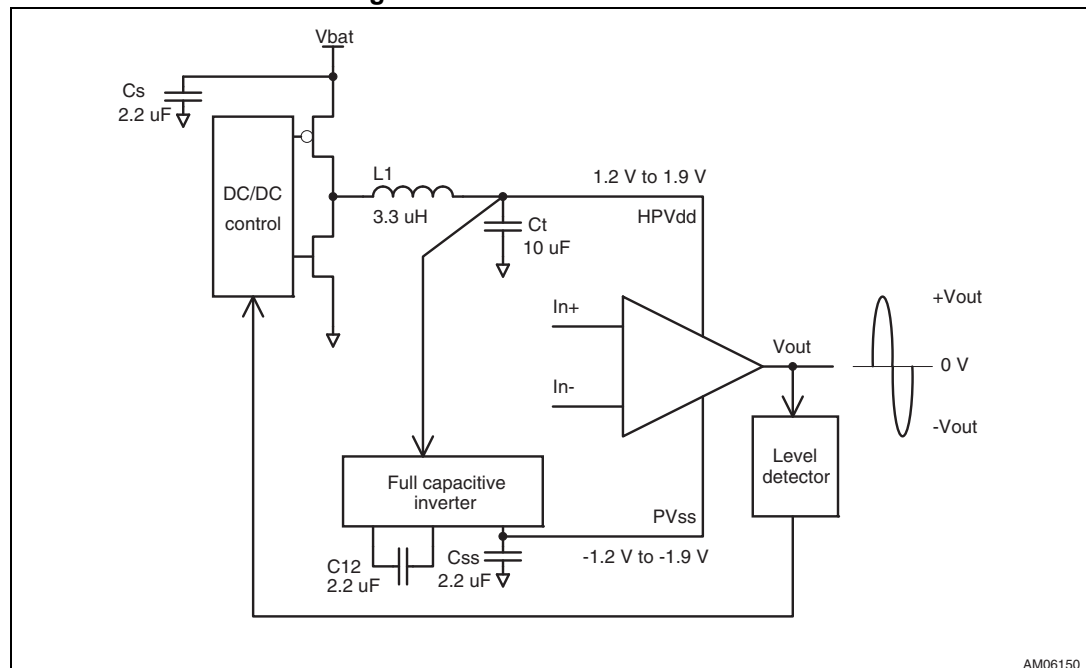
Figure 64. A22H165 architecture
