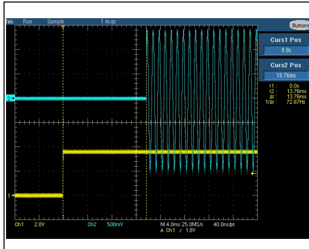
Figure 62. Wake-up time
