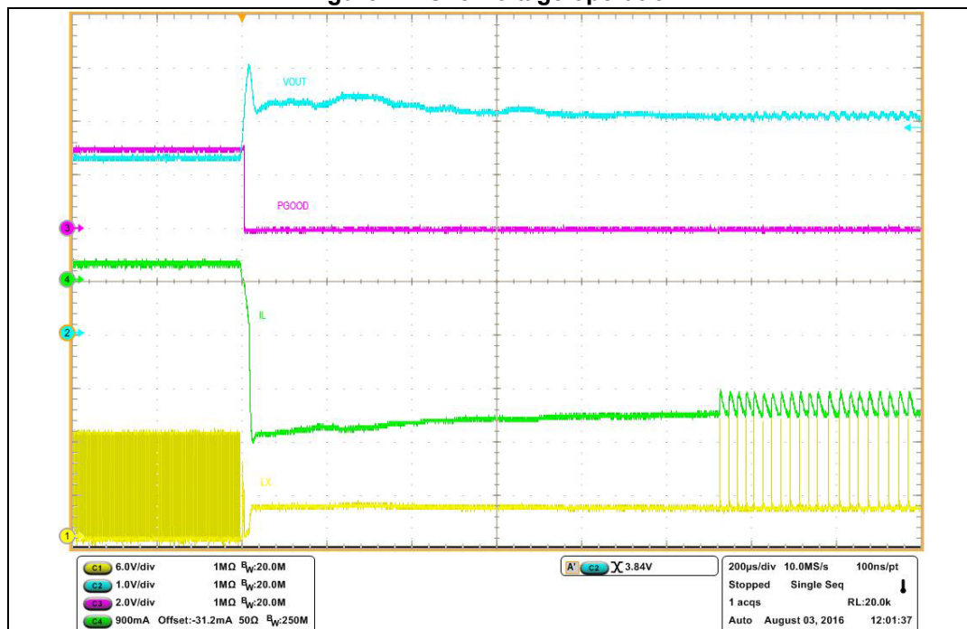
Figure 27. Overvoltage operation
