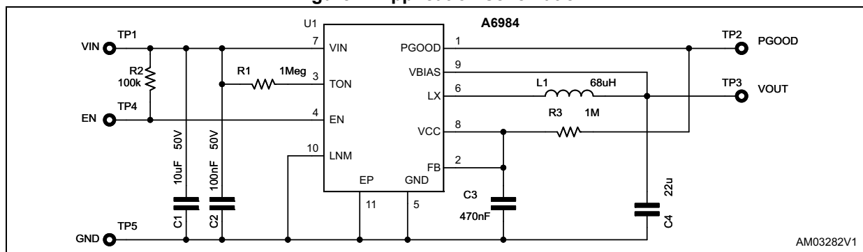
Figure 1. Application schematic
