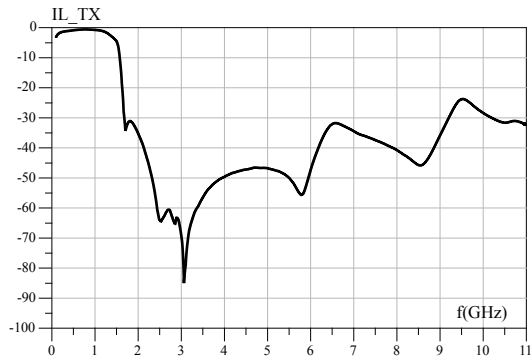
Figure 5. Transmission wide band with harmonics attenuation (dB)
